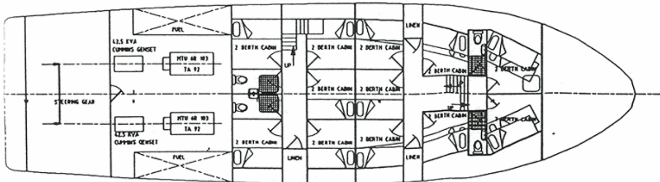
PLAN BELOW MAIN DECK
