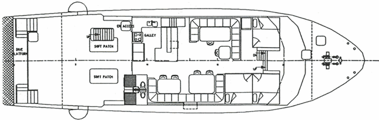
PLAN ON MAIN DECK
